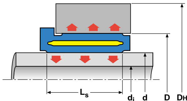
Principle built-in of an ETP connection.
