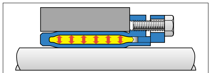
When the screws have been tightened ETP-CLASSIC will create an even surface pressure against the hub and shaft along virtually the entire length.
