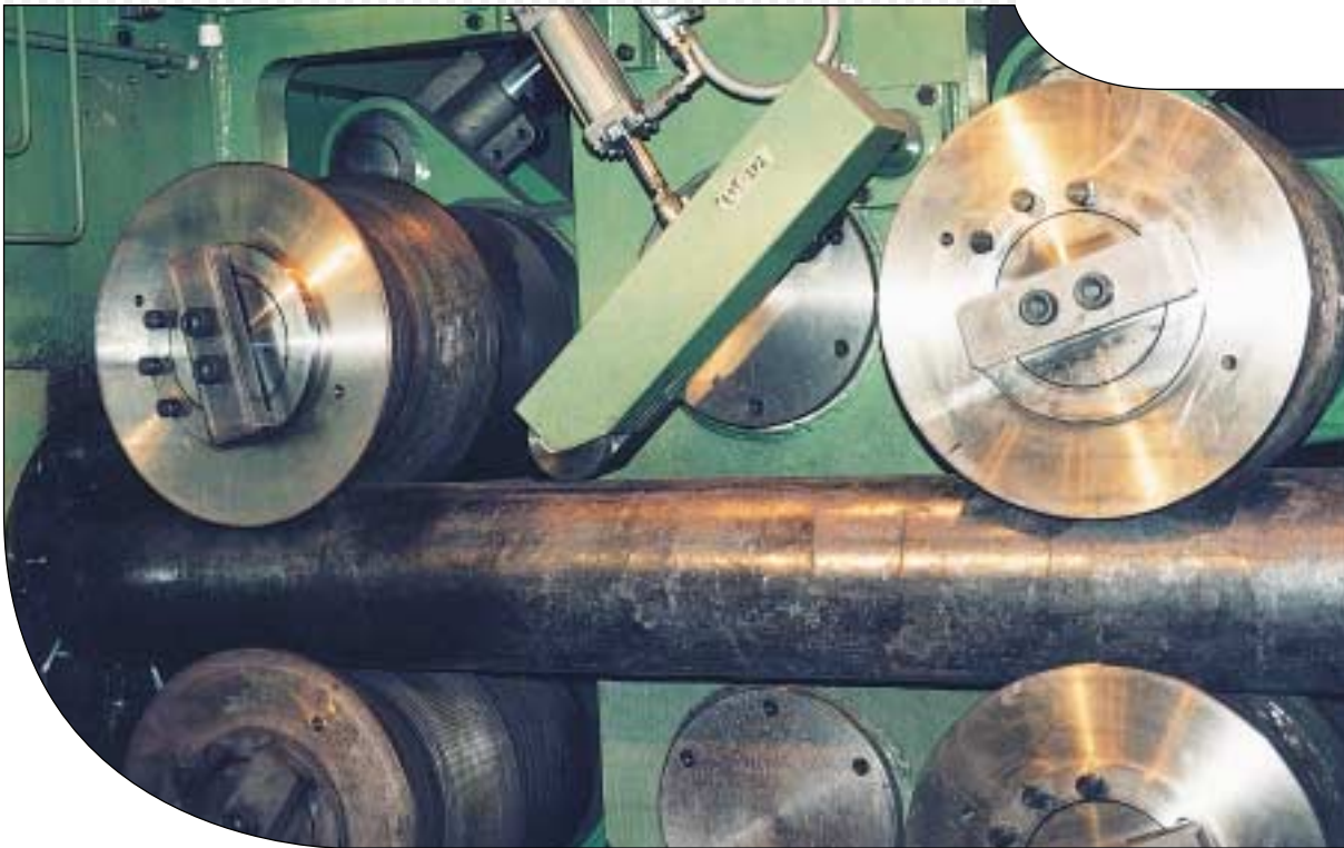
ETP-HYLOC, due to its robust design, is ideally suited to work in difficult environments and heavy operations like steel rolling mills, process industry etc. An interesting application, among many, has been fastening of rolls to shafts. ETP-HYLOC is fast to mount, has good concentricity and can take high radial loads.
