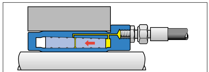
Dismantling: Apply pressure in the "OFF" and "P" (not shown) connections. ETP-HYLOC returns to its original measurements and the joint is loose.
