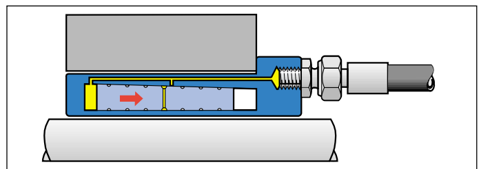
Mounting: Apply pressure in the "ON" and "P" (not shown) connections. When mounted no hydraulic pressure remains. The small conical angle prevents the piston from releasing.
